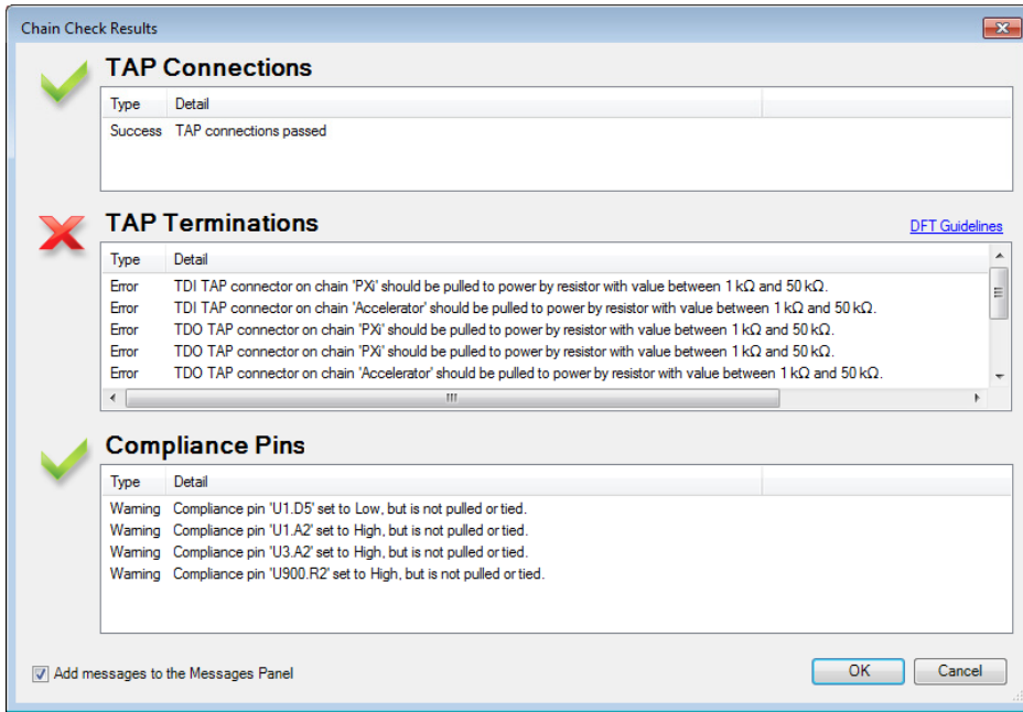
The XJTAG Chain Checker identifies and categorizes faults and warnings in the boundary scan chain(s)
