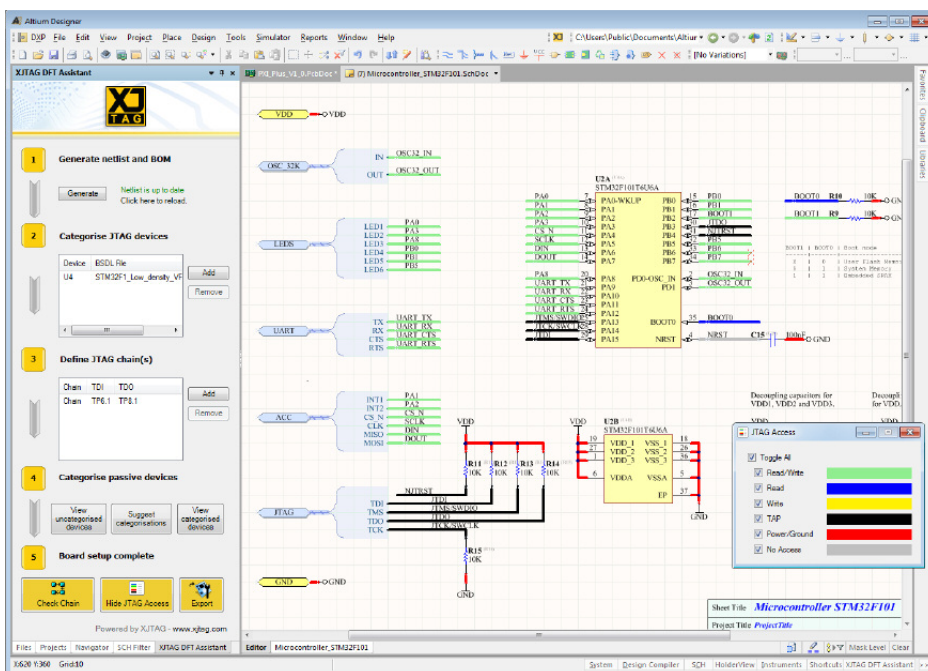
The XJTAG Access Viewer provides a clear indication of test access at any point during design
